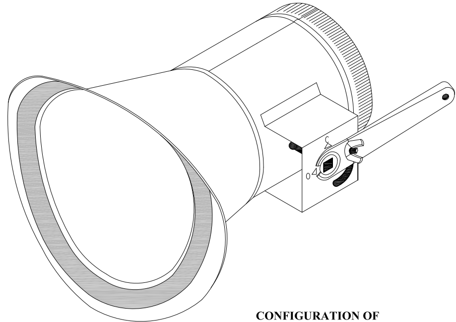
CONFIGURATION OF 14" THROUGH 20" DIAMETERS
